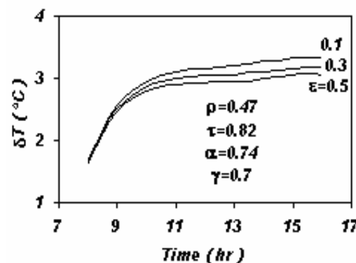
Fig. 9-Effects of tube emissivity on the oil temperature
